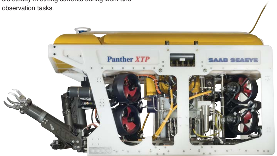
SAAB SEAEYE'S HIGH PERFORMANCE, LIGHT WORK ROV
