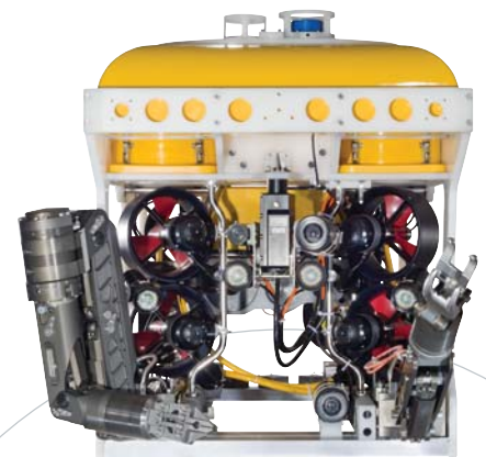
SAAB SEAEYE'S HIGH PERFORMANCE, LIGHT WORK ROV
